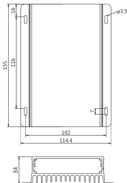
MES200 dimensions: Overall dimensions: 155 \times 114.4 \times 34 mm Mounting dimensions: 116 \times 102 mm Mounting hole diameter: \phi 3.5 mm
