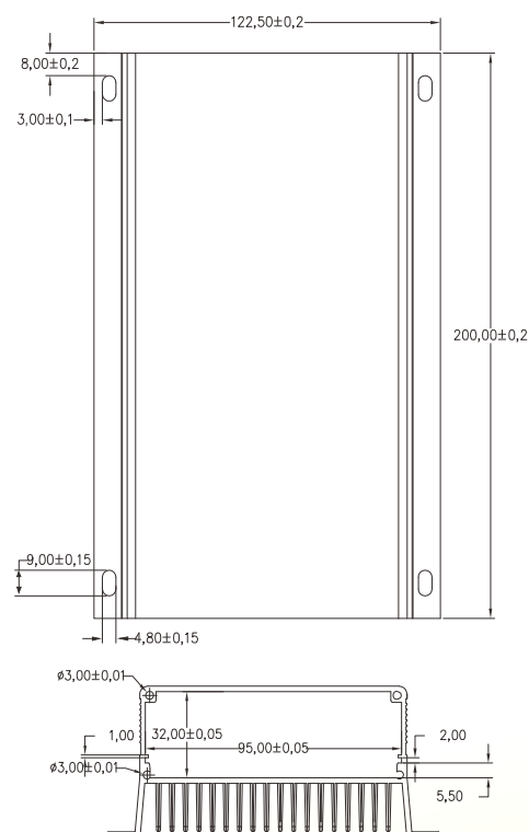
MES260/MES300 dimensions: Overall dimensions: 200 \times 122.5 \times 56 mm Mounting dimensions: 175 \times 113 mm Mounting hole diameter: \phi 3.5 mm
