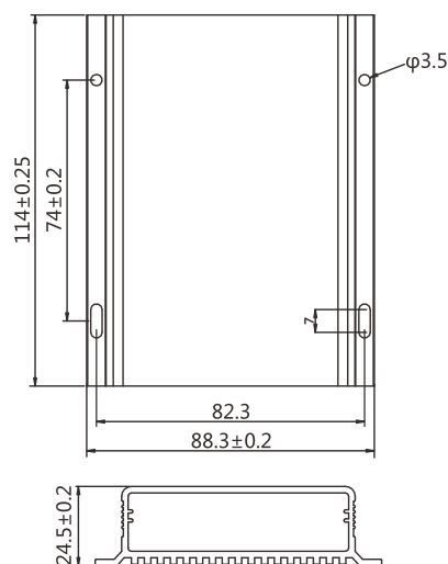
MES80/120 dimensions: Overall dimensions: 114 \times 88.3 \times 24.5 mm Mounting dimensions: 74 \times 82.3 mm Mounting hole diameter: \phi 3.5 mm
