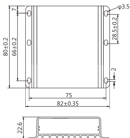
MES60 dimensions: Overall dimensions: 80 \times 82 \times 22.6 mm Mounting dimensions: 66 \times 75 mm Mounting hole diameter: \phi 3.5 mm
