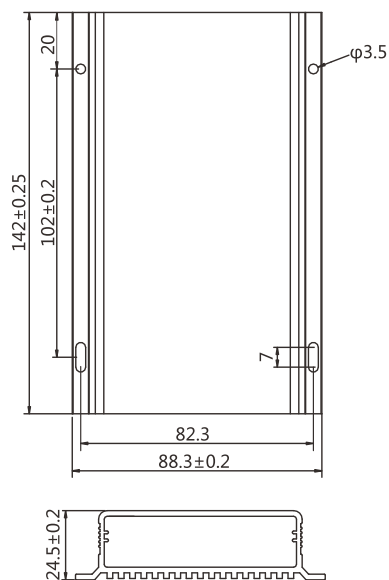
MES160 dimensions: Overall dimensions : 142 \times 88.3 \times 24.5 mm Mounting dimensions: 102 \times 82.3 mm Mounting hole diameter: \phi 3.5 mm
